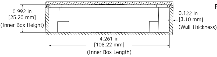
SECTION B-B Side View of Assembly
