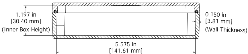
SECTION B-B Side View of Assembly
