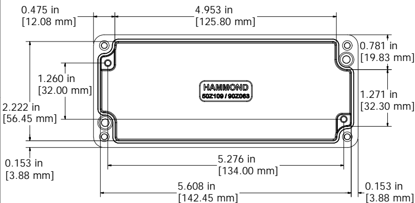
Top View Looking Inside Box
