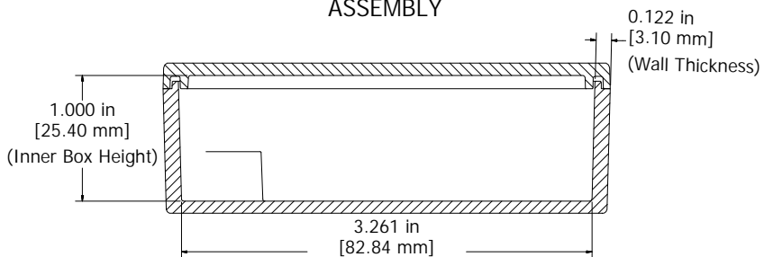
SECTION E-E Side View of Assembly
