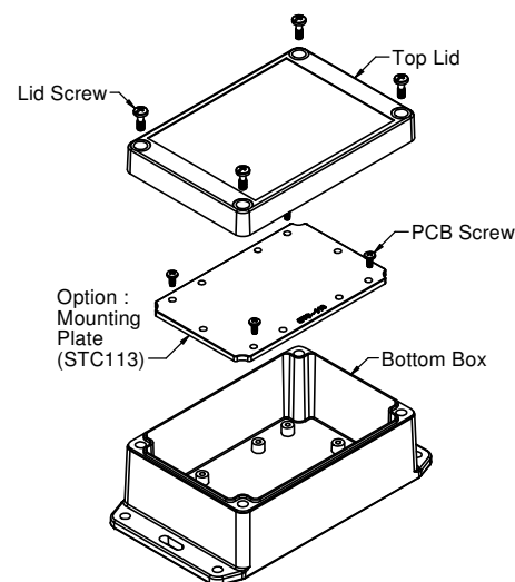
Exploded view
