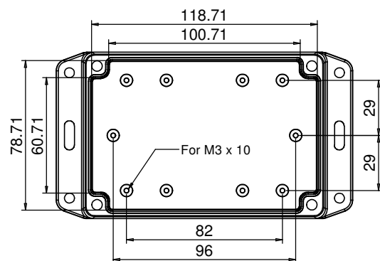
Inner view
