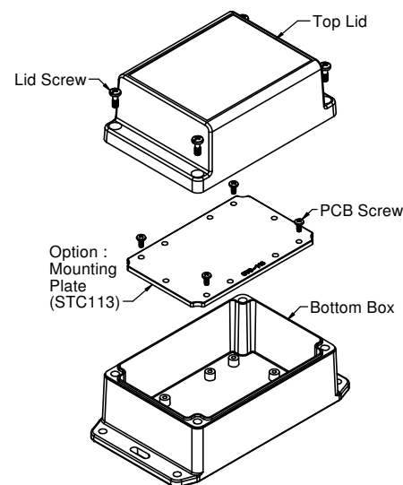
Exploded view
