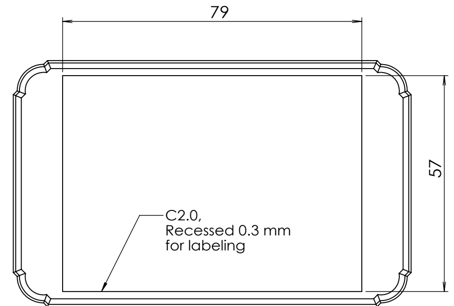
BOTTOM view
