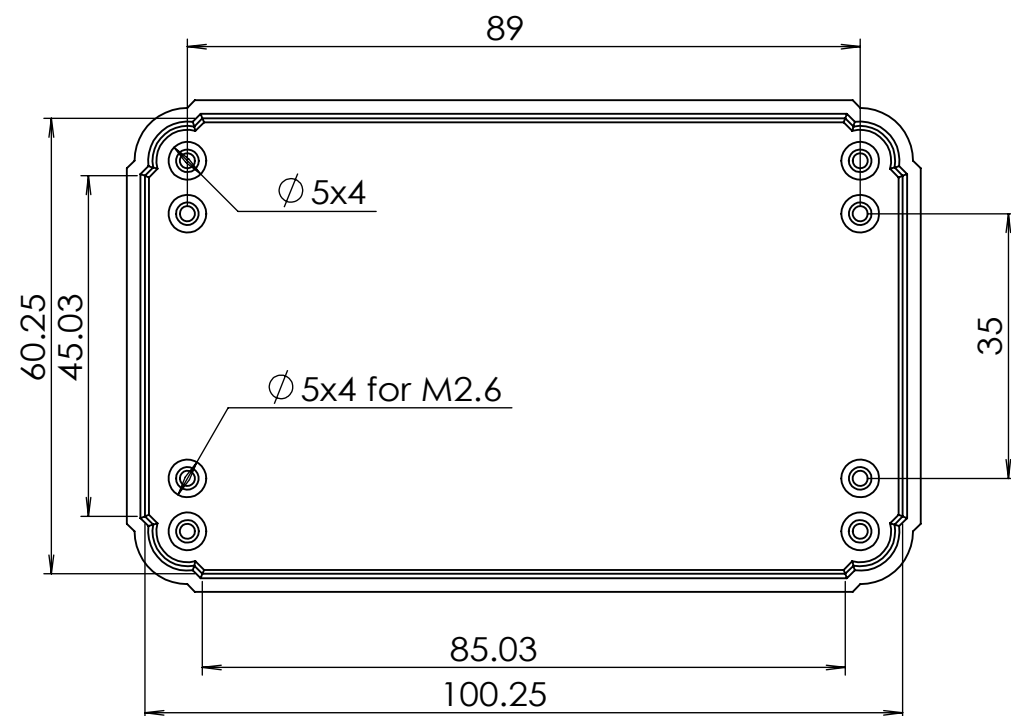
INNER view
