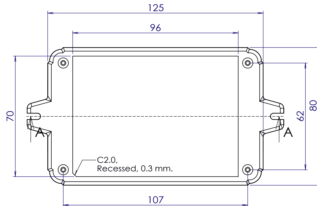
Top view
