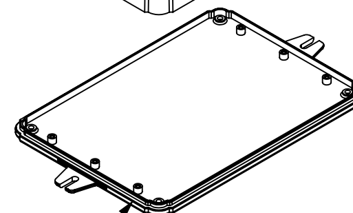
Flange Cover-
